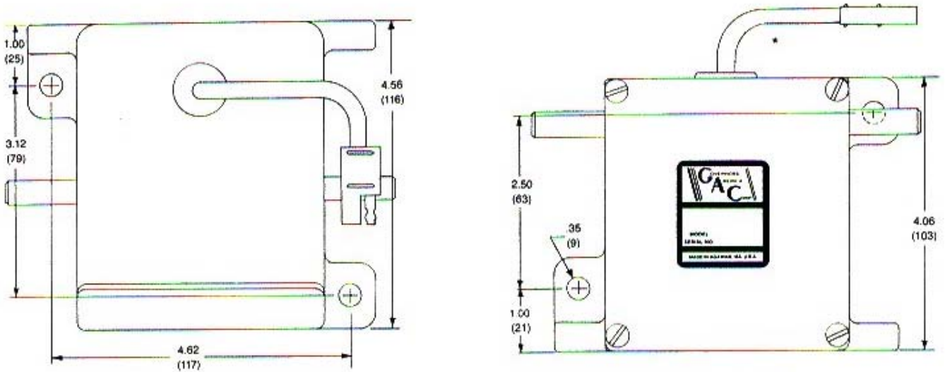
ADB and ADC Actuator Outline Dimensions
